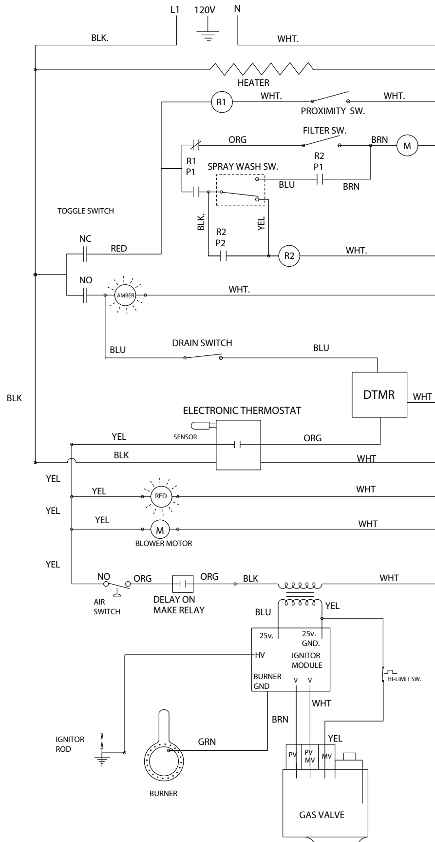
PAR-3-HE GAS FRYER W/ DTMR CONTROL
