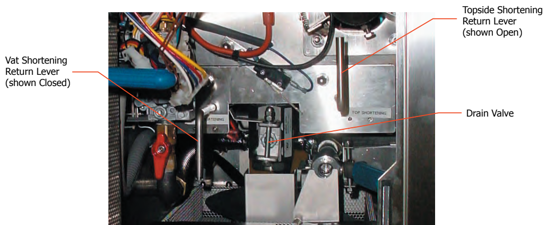
18" PAR-3-HE GAS FRYER
