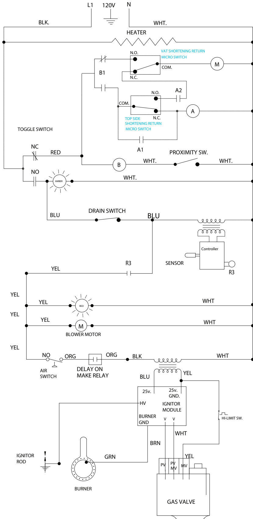
PAR-3-HE GAS FRYER W/ COMPUTER
