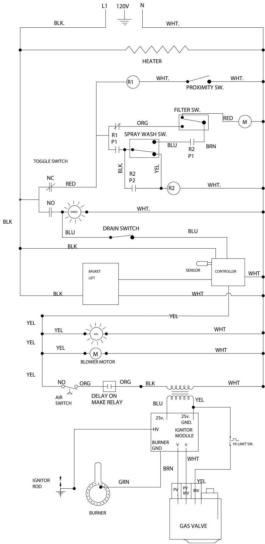
PAR-3-HE GAS FRYER W/ COMPUTER & BASKET LIFT
