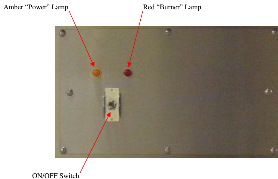
CONTROL PANEL
